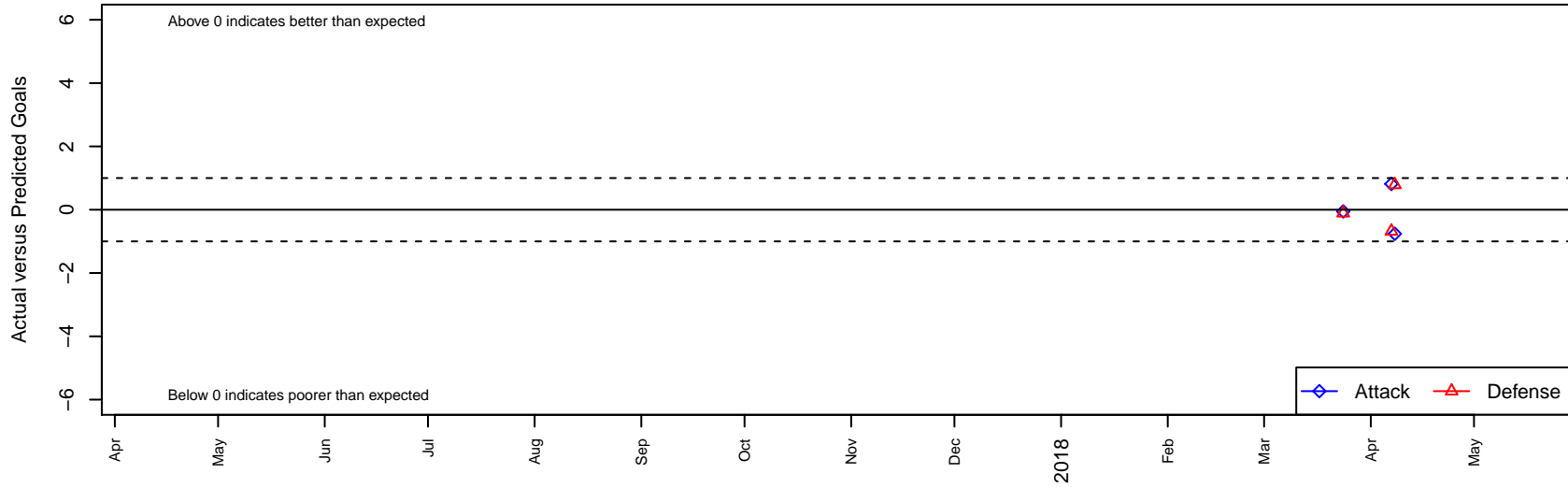
Quad City Fusion G00 Dots are actual minus expected GF (blue circles) and GA (red triangles). Blue line is smoothed change in attack strength. Red is smoothed change in defense strength.
